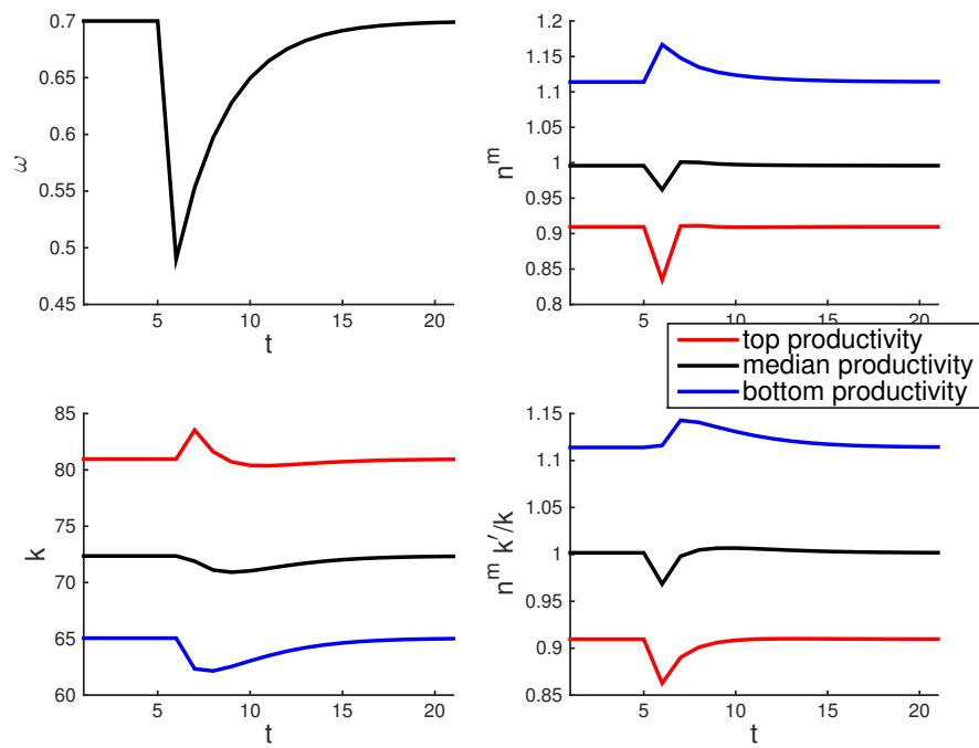
Figure 7: Training decisions on the transition path of the basic model when financing constraint is binding.
