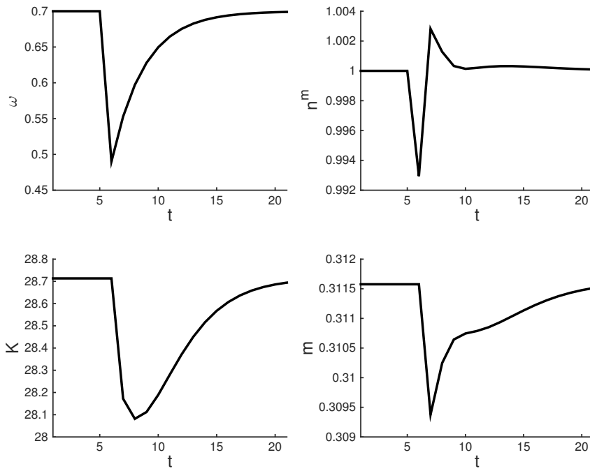
Figure 6: Dynamics in the basic model when financing constraint is not binding.
